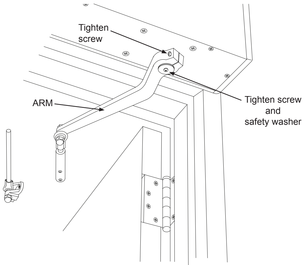
Arm placement in full open position
