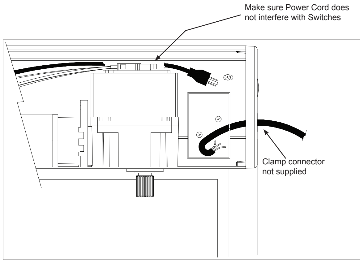
120 vAC RMS to Controller Module connection
