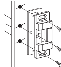
3. DRILL 7/32 " HOLE, TAP 1/4 "-20P THREAD
