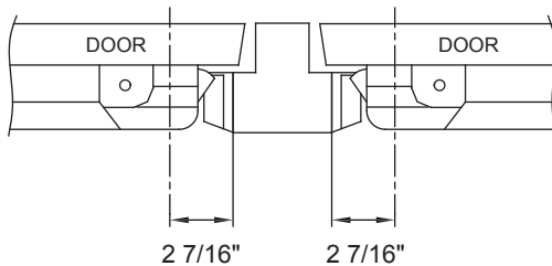
B. DOUBLE DOOR WITH MULLION
